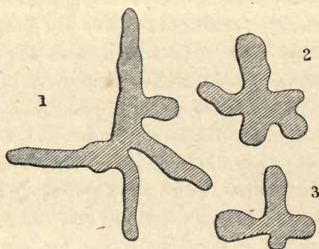
Sections of trunk of a Bornean Forest-tree.
