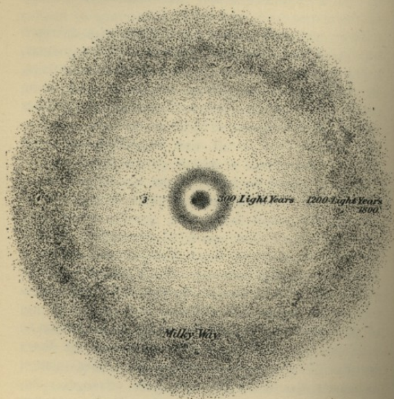
DIAGRAM OF STELLAR UNIVERSE (Plan).
