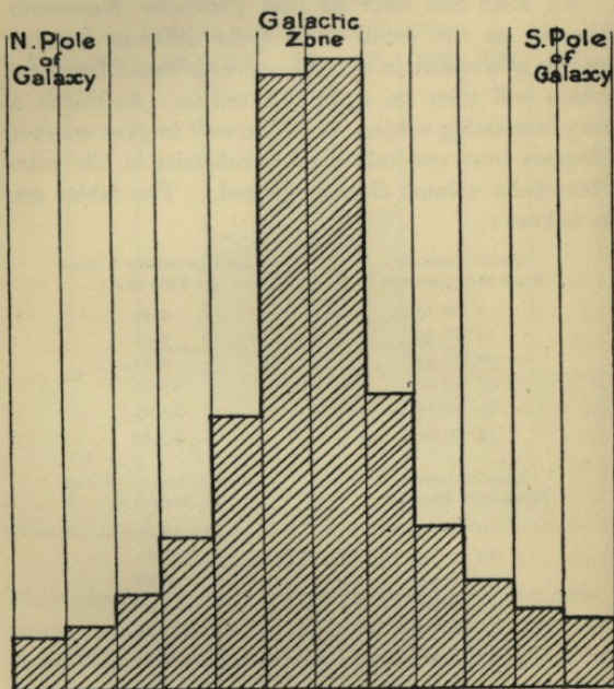
DIAGRAM OF STAR-DENSITY.
