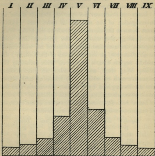
DIAGRAM OF STAR-DENSITY
